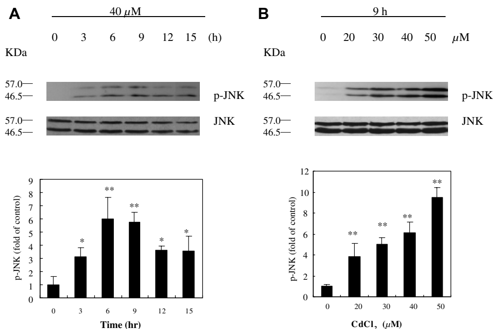
Fig. 3. Effects of cadmium on phosphorylation of JNK in LLC-PK 1 cells. (A) Time course of cadmium-induced accumulation of phosphorylated JNK. LLC-PK 1 cells were exposed to 40 μM cadmium for 0–15 h. (B) Dose effects of cadmium on the accumulation of phosphorylated JNK. LLC-PK 1 cells were incubated with 20–50 μM cadmium for 9 h, and proteins (50 μg) prepared from whole cell extracts were analyzed by western blot using phospho-specific JNK antibody (upper panel) or phosphorylation state-independent JNK antibody (lower panel). Densitometric analysis of the phosphorylated JNK and total JNK protein was calculated from the average of three experiments. Each value was expressed as the ratio of phosphorylated JNK level to total JNK level, and the value of control was set to 1. Each column and bar represents mean ± SD. * Indicates significant difference compared to control group at p < 0.05 analyzed using one-way ANOVA test.
