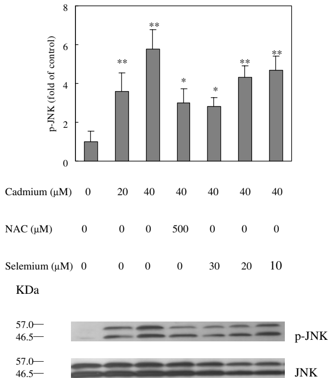
Fig. 4. Effects of selenium on the cadmium-induced JNK phosphorylation. LLC-PK 1 cells were pre-incubated with 500 \mu\text{M} NAC or 10, 20, 30 \mu\text{M} selenium for 30 min, then treated with 40 \mu\text{M} cadmium for 9 h, phosphorylation of JNK was analyzed by the Western blot. Densitometric analysis of the phosphorylated JNK and total JNK protein was calculated from the average of three experiments. Each value was expressed as the ratio of phosphorylated JNK level to total JNK level, and the value of control was set to 1. Each column and bar represents mean \pm SD. *Indicates significant difference compared to control group at p < 0.05 analyzed using one-way ANOVA test.
