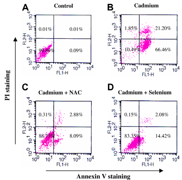
Fig. 2. Inhibition of cadmium-induced apoptosis by selenium and N -acetyl-L-cysteine (NAC). The LLC-PK 1 cells were treated with 40 \mu M cadmium for 12 h or pretreated with 500 \mu M NAC or 20 \mu M selenium for 30 min, then exposed to 40 \mu M cadmium for 12 h, cell distribution was analyzed with Annexin V/FITC and propidium iodide (PI) uptake. The FITC and PI fluorescence measured using flow cytometer with FL-1 and FL-2 filters, respectively. LL, living cells (Annexin V negative/PI negative); LR, early apoptotic/primary apoptotic cells (Annexin V positive/PI negative); UR, late apoptotic/secondary apoptotic cells (Annexin V positive/PI positive); UL, necrotic cells (Annexin V negative/PI positive). Numbers in the respective quadrant profiles indicate the percentage of the cells present in this area.
