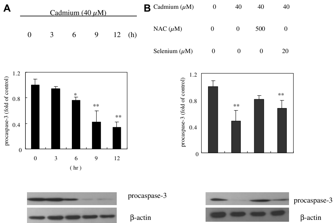
Fig. 5. (A) Cadmium-induced procaspase-3 activation in LLC-PK 1 cells. The cells were incubated with 40 \mu M cadmium for the indicated times. The cells were harvested and lysed. 50 \mu g of protein lysate was subjected to 12% SDS-PAGE gel and then immunoblotted with procaspase-3 antibodies. \beta -Actin was used as loading control. (B) Effects of selenium on cadmium-induced procaspase-3 activation in LLC-PK 1 cells. Cells were pretreated with 500 \mu M NAC and 20 \mu M selenium for 30 min and then incubated with 40 \mu M cadmium for 9 h. The cells were harvested and lysed. 50 \mu g of protein lysate was subjected to 12% SDS-PAGE gel and then immunoblotted with procaspase-3 antibodies. \beta -Actin was used as a loading control. Densitometric analysis of procaspase-3 protein was calculated from the average of three experiments. Each value was expressed as the ratio of procaspase-3 level to \beta -actin level, and the value of control was set to 1. Each column and bar represents mean \pm SD. *Indicates significant difference compared to control group at p < 0.05 analyzed using one-way ANOVA test.
