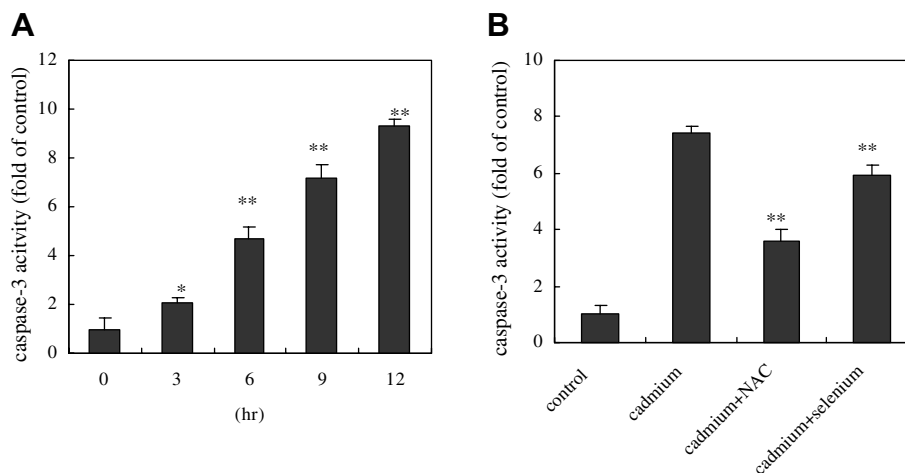
Fig. 6. (A) Cadmium-induced caspase-3 activation in LLC-PK 1 cells. The cells were incubated with 40 \mu M cadmium for 0–12 h. Data are the means \pm SD. * p < 0.05 compared with control group. (B) Effects of selenium and NAC on cadmium-induced caspase-3 activation. The LLC-PK 1 cells pre-treated with 500 \mu M NAC and 20 \mu M selenium for 30 min, then incubated with 40 \mu M cadmium for 9 h. Data are the means \pm SD. * p < 0.05 compared with cadmium treatment group. The relative activities of caspase-3 shown are calculated from the average of three experiments. Each value was expressed as the ratio of caspase-3 activation level to control level, and the value of control was set to 1.
