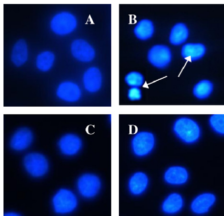
Fig. 1. Effects of selenium on cadmium-induced LLC-PK 1 cells apoptosis by Hoechst 33258 staining. (A) In controls, the majority of cells had uniformly stained nuclei. (B) After exposure to 40 \mu M cadmium for 12 h showed morphological changes typical of apoptosis (i.e. nuclei fragmentation with condensed chromatin). (C) Cells pre-treated with 500 \mu M NAC for 30 min, then exposed to 40 \mu M cadmium for 12 h, the apoptosis cells have been clearly decreased compared to cadmium treatment groups. (D) Cells pre-treated with 20 \mu M selenium for 30 min, then exposed to 40 \mu M cadmium for 12 h, the apoptosis cells have also been observed to drop compared to cadmium treatment groups.
